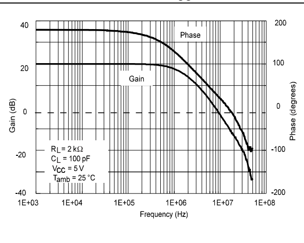
Figure 2. Voltage gain and phase vs. frequency V_{CC} = 5\text{ V}
