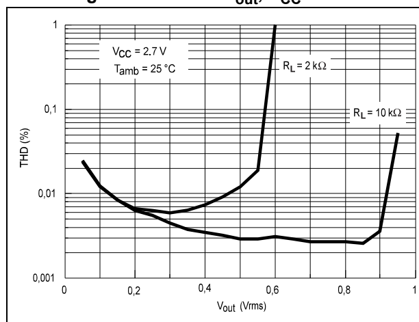
Figure 5. THD vs. V_{out} , V_{CC} = 2.7\text{ V}
