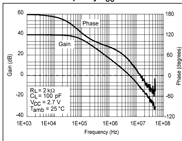
Figure 3. Voltage gain and phase vs. frequency V_{CC} = 2.7\text{ V}
