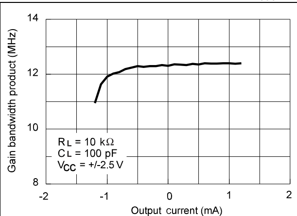
Figure 8. Gain bandwidth product vs. I_{out}
